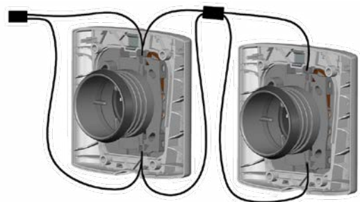
Wall inlet parallel connection.
