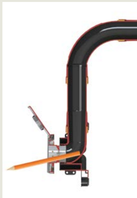
The sharpest elbow in the entire piping system is located directly behind the wall inlet. It prevents long items such as pencils from entering the piping system.
